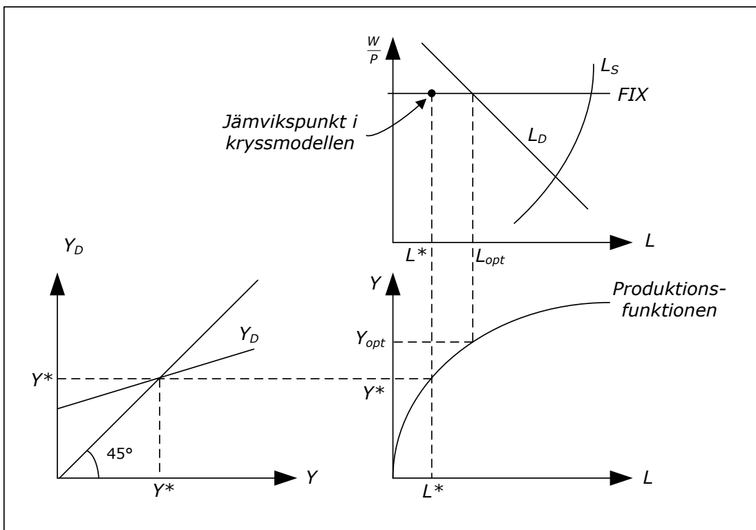
Fig. 11.8: Determination of L in the cross model.
