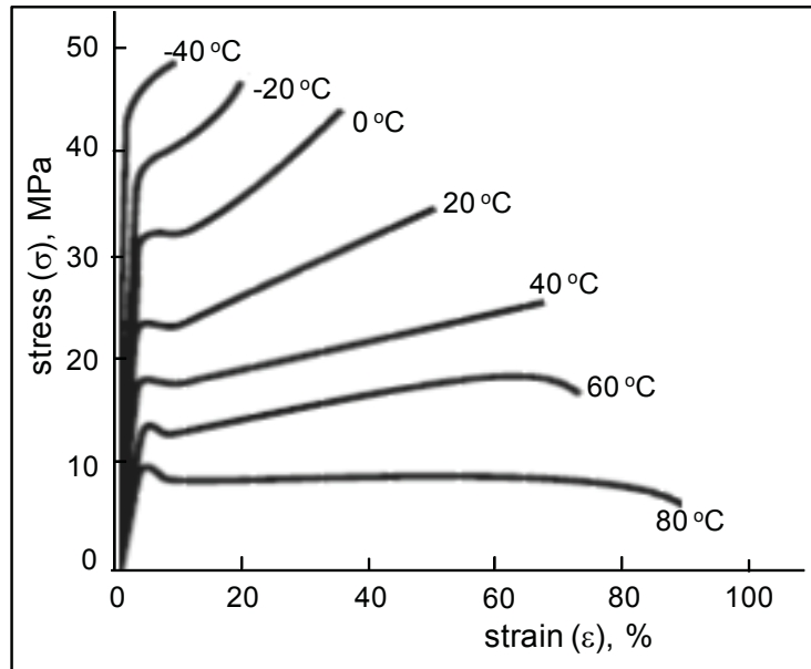
Figure 6.7 Stress-strain curves for HIPS at a range of temperatures from -40\text{ }^{\circ}\text{C} to 80\text{ }^{\circ}\text{C} (tests conducted at 2 mm/min cross-head speed) (source: Ehrenstein (2001, p182))
