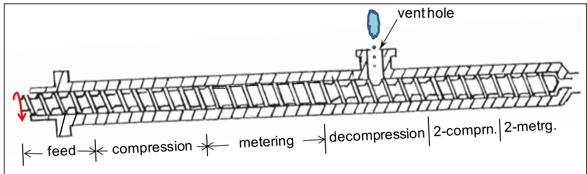
Figure 3.20 Features of a vented extruder
